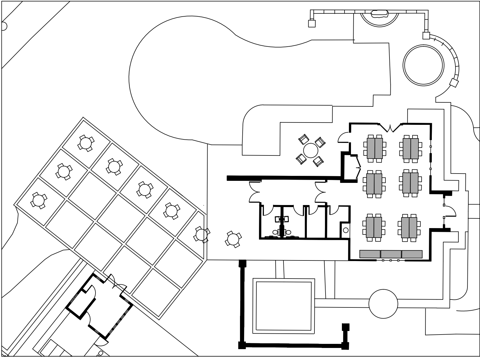
Hunziker House Standard, 48 seated
